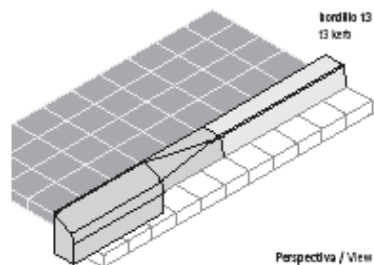
Perspectiva / View
