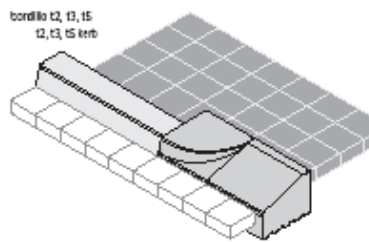
View / Perspectiva
